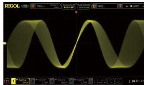
Changes of each frame of waveforms of the sweep signal can be clearly observed in the highly refresh mode.
